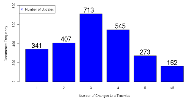
Figure 3: Number of changes to TimeMaps.
