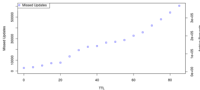
Figure 8: Number of missed cache replacements by TTL value.
