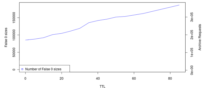
Figure 9: False 0-sized TimeMaps by TTL value for conditional .
