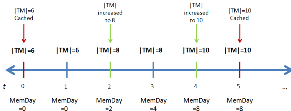
Figure 7: MemDay calculation example.
